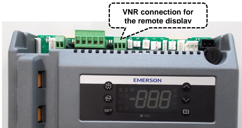
Figure 12: VNR connection for the remote display
