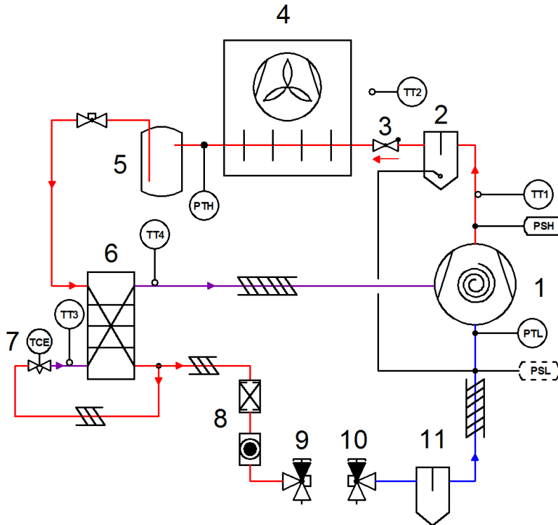
Figure 4: P&I diagram for ZXLE units
