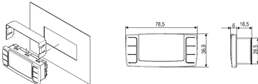
Figure 11: Remote display front panel mounting
