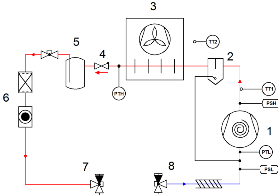
Figure 5: P&I diagram for ZXDE units
