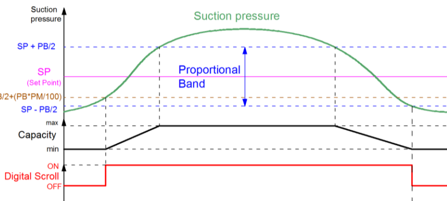
Figure 14: Digital operation
