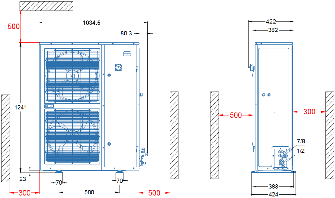
Figure 24: Fixing dimensions and distances – Dual-fan unit
