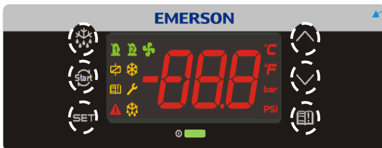
Figure 10: Local display
