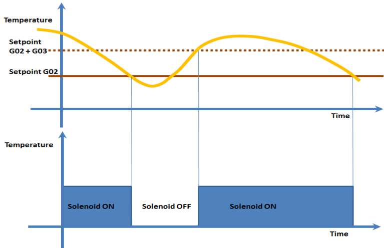
Figure 13: Pump-down functionality with temperature sensor
