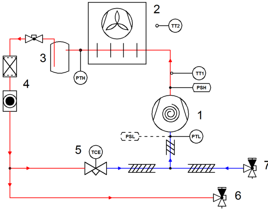
Figure 3: P&I diagram for ZXME units
