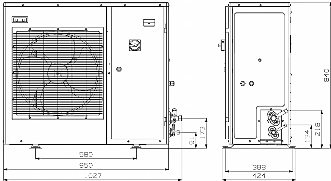
Figure 17: Dimensions of models ZXME020E, ZXME025E, ZXME030E & ZXME040E and models ZXLE020E, ZXLE030E & ZXLE040E (single-fan units)
