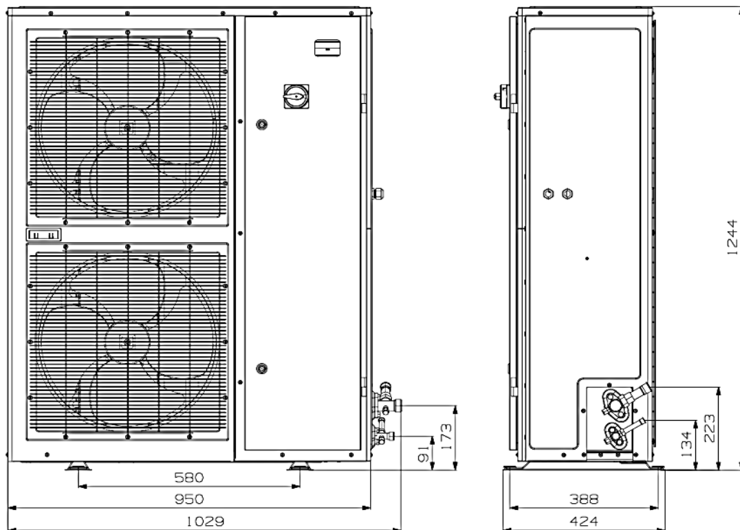
Figure 18: Dimensions of models ZXME050E, ZXME060E, ZXME075E, ZXDE040E, ZXDE050E, ZXDE060E, ZXDE075E, ZXLE050E, ZXLE060E & ZXLE075E (dual-fan units)
