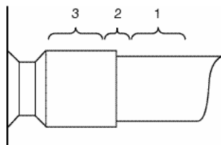
Figure 22: Suction tube brazing areas
